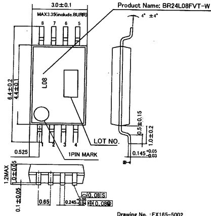
Fig.-4(d) PHYSICAL DIMENSION TSSOP-B8 (BR24L08FVT-W)
