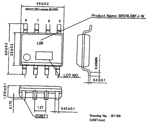
Fig.-4(b) PHYSICAL DIMENSION SOP-J8 (BR24L08FJ-W)
