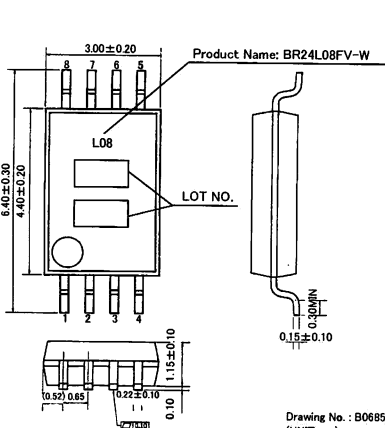
Fig.-4(c) PHYSICAL DIMENSION SSOP-B8 (BR24L08FV-W)
