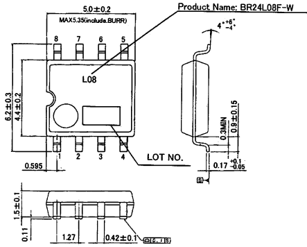
Fig.-4(a) PHYSICAL DIMENSION SOP8 (BR24L08F-W)
