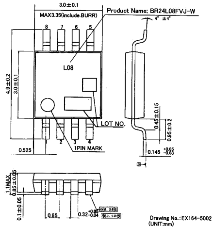
Fig.-4(f) PHYSICAL DIMENSION TSSOP-B8J (BR24L08FVJ-W)
